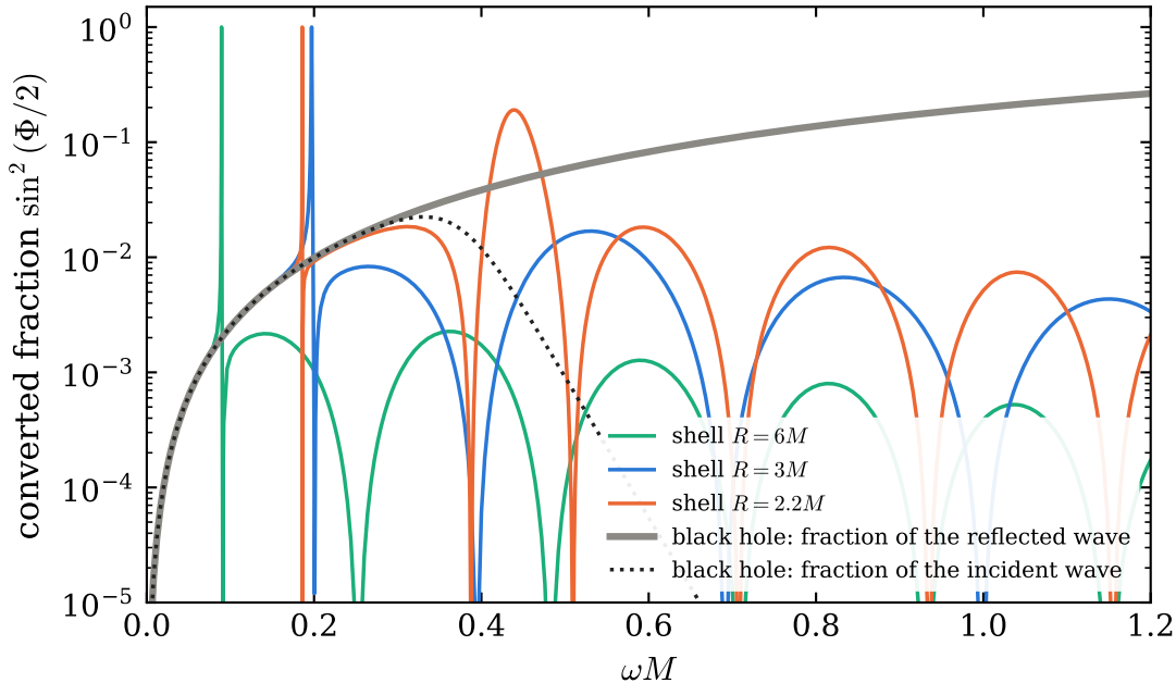
Polarization conversion on reflection ( \ell = 2 , incident at 45^\circ to the E/B axes)
